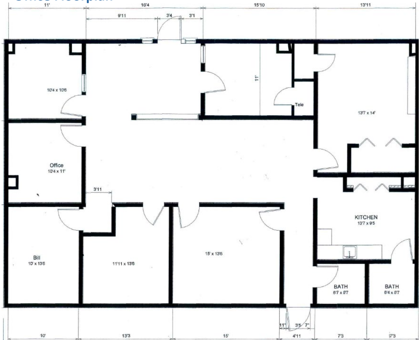
Office Floorplan
