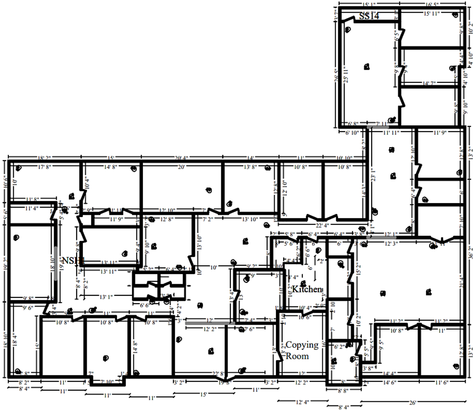
Floor Plan
